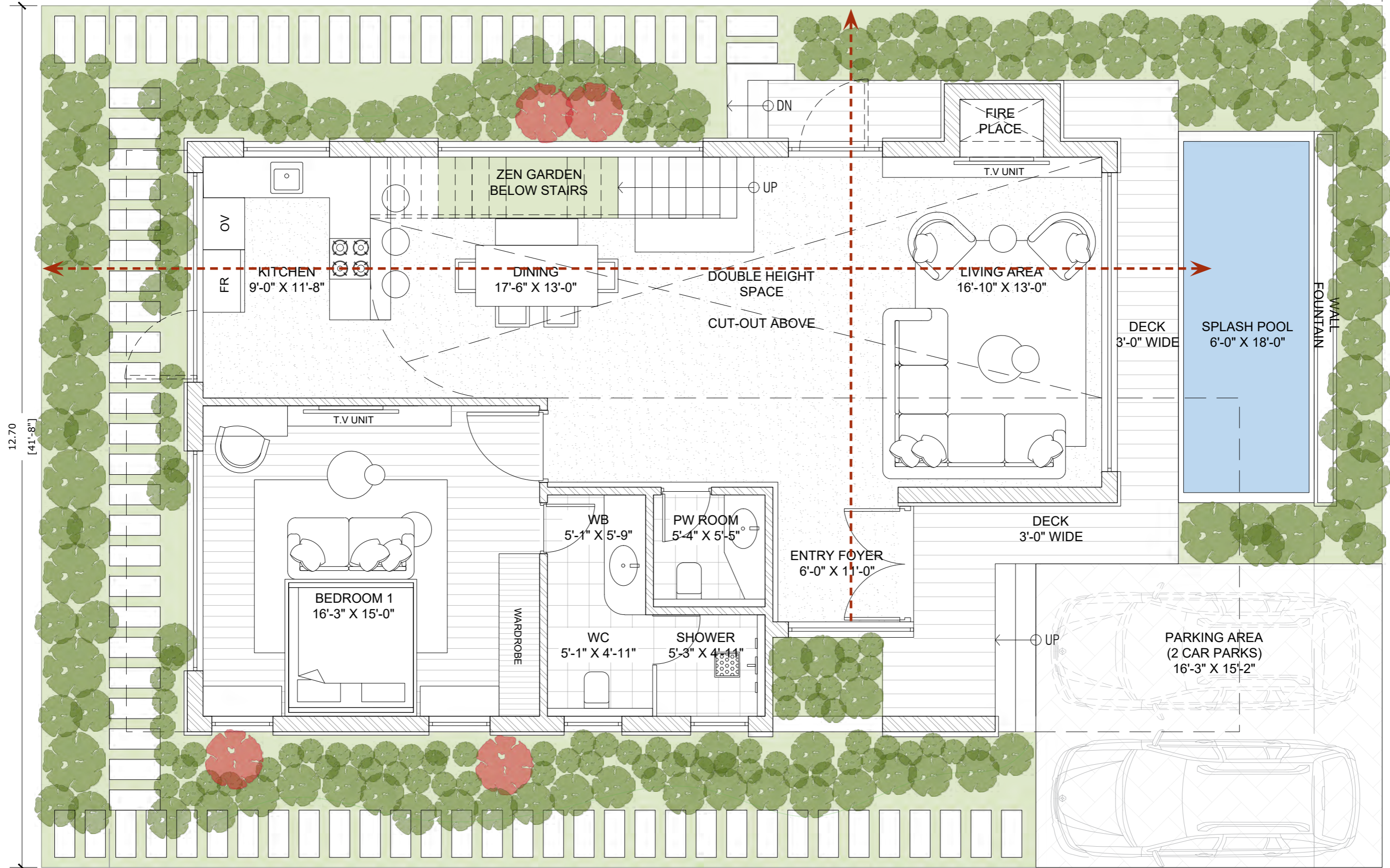
Ground Floor Area - 133.75 sqm; 1440sqft
